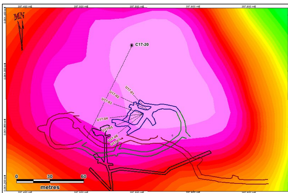
Figure 9.20 Mise-a-la-Masse Survey
