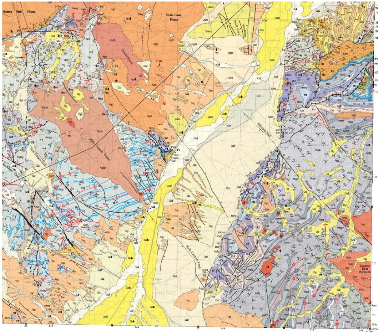
Figure 7.1 Regional Geology
