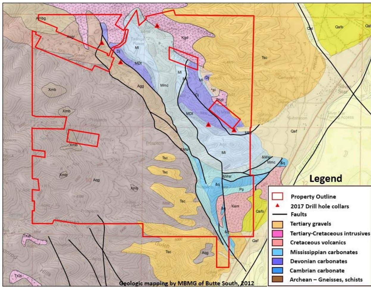
Figure 7.2 Property Geology
